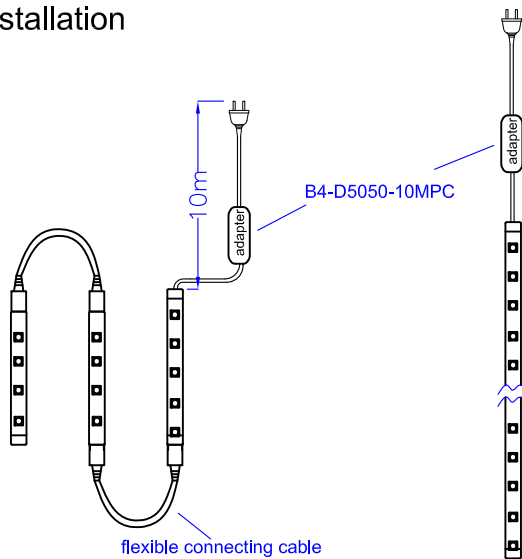
Curve installation
